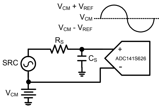
Figure 5 – Single-Ended Input
