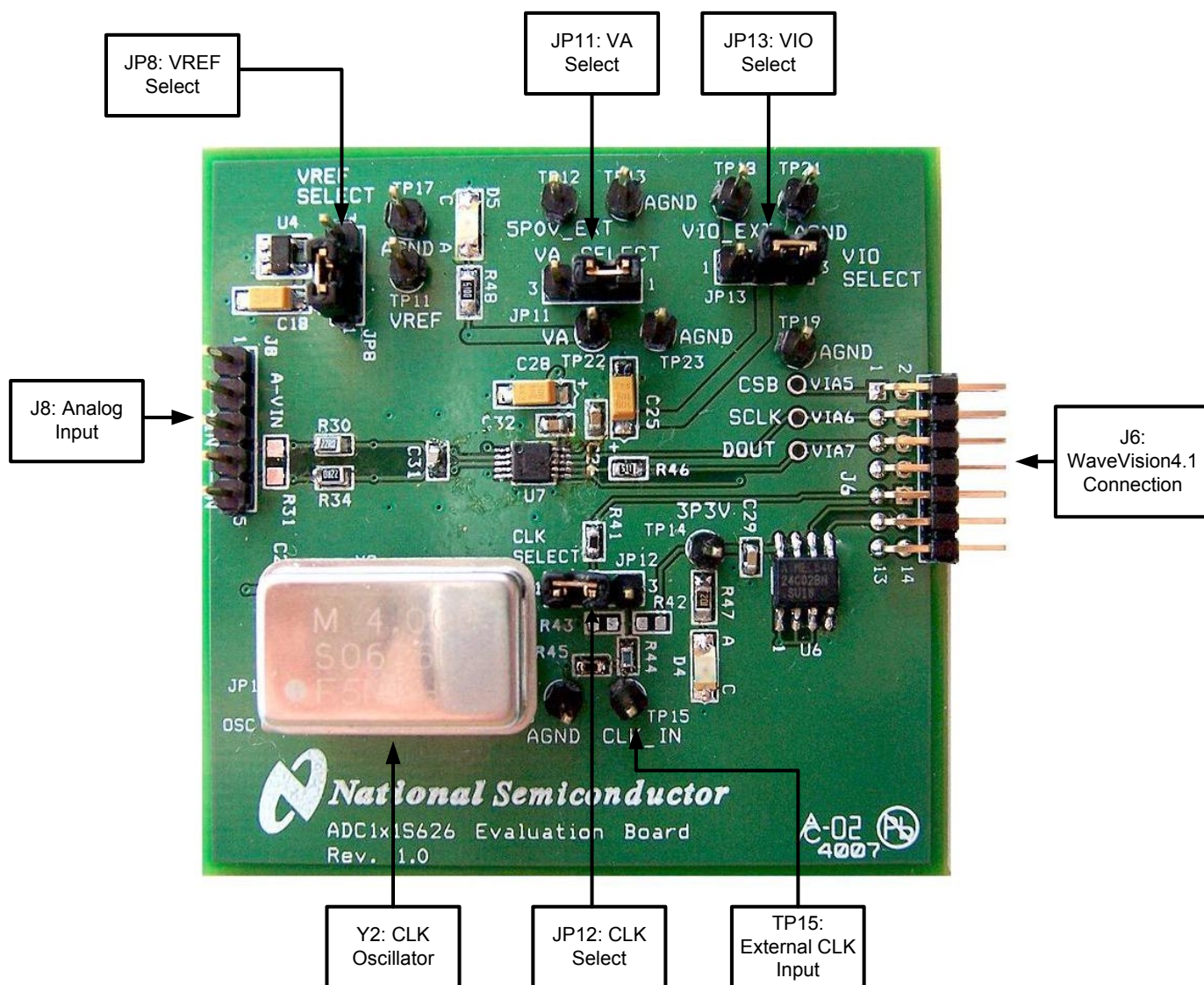
Figure 1 – Components Locations
